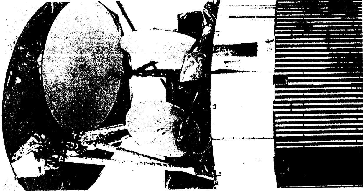
October 28: The first Intelsat V1 satellite launched and placed in orbit over the Atlantic Ocean.
