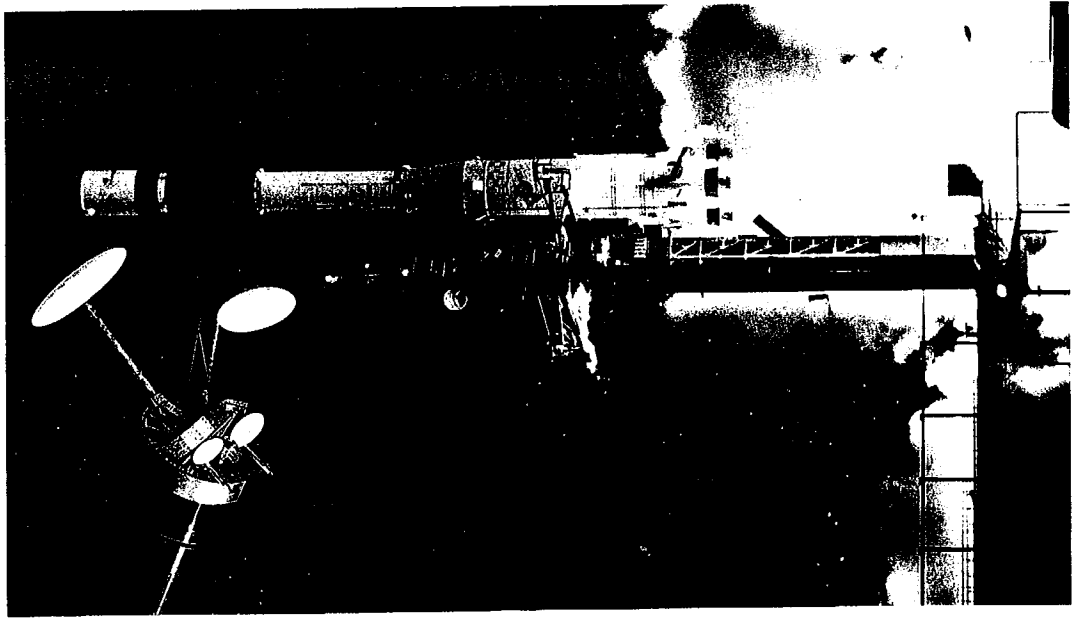
October 28: The first Intelsat V1 satellite launched and placed in orbit over the Atlantic Ocean.
